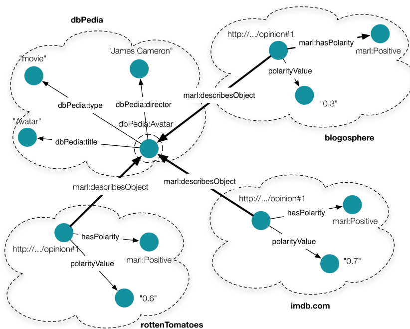
Fig. 6. Sample RDF graph with opinions linked indirectly via metadata references to common entities.
